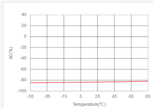
Bias TCC Characteristics LCR meter, 1000kHz, 1Vms, 12.5Vdc
