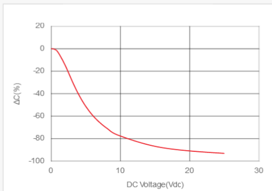
DC Bias Characteristics LCR meter, 1000kHz, 1Vms
