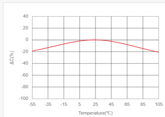
Temperature Characteristics of Capacitance(TCC) LCR meter, 1kHz, 0.15Vrms
