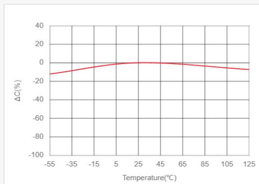
Temperature Characteristics of Capacitance(TCC) LCR meter, 1kHz, 0.35Vrms
