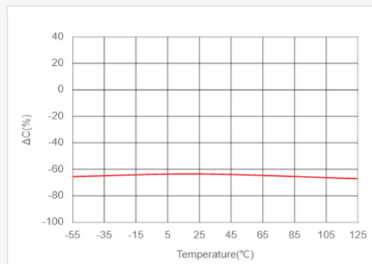
Bias TCC Characteristics LCR meter, 1kHz, 1Vrms, 37.5Vdc
