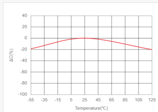
Temperature Characteristics of Capacitance(TCC) LCR meter, 1kHz, 0.005Vrms
