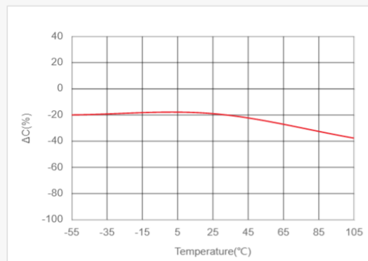
Bias TCC Characteristics LCR meter, 1kHz, 0.5Vrms, 1.25Vdc
