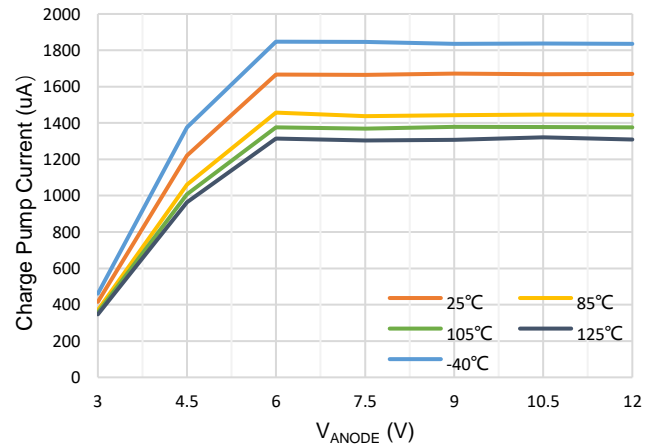
Figure 3. Charge Pump Current vs V_{ANODE} at V_{CAP}= 6\text{ V}
