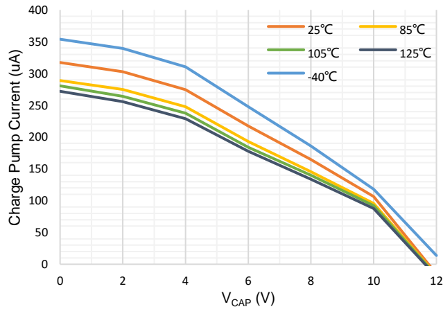
Figure 4. Charge Pump V-I at V_{ANODE} \geq 12\text{V}
