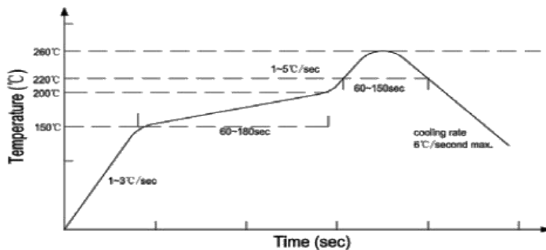
Reflow -curve
