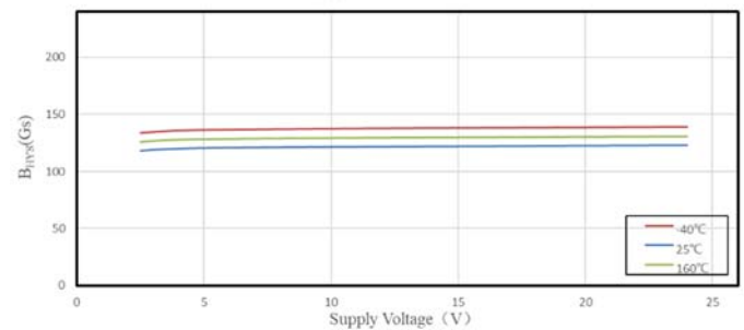
SC2446 B HYS VS. Supply Voltage
