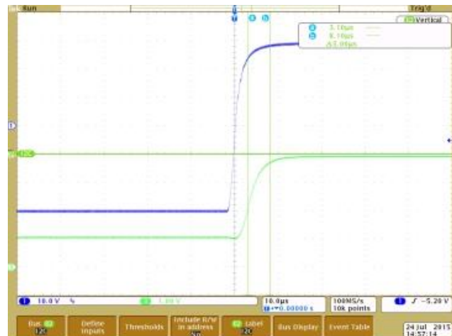
Figure 6. < 5uS Response Time
