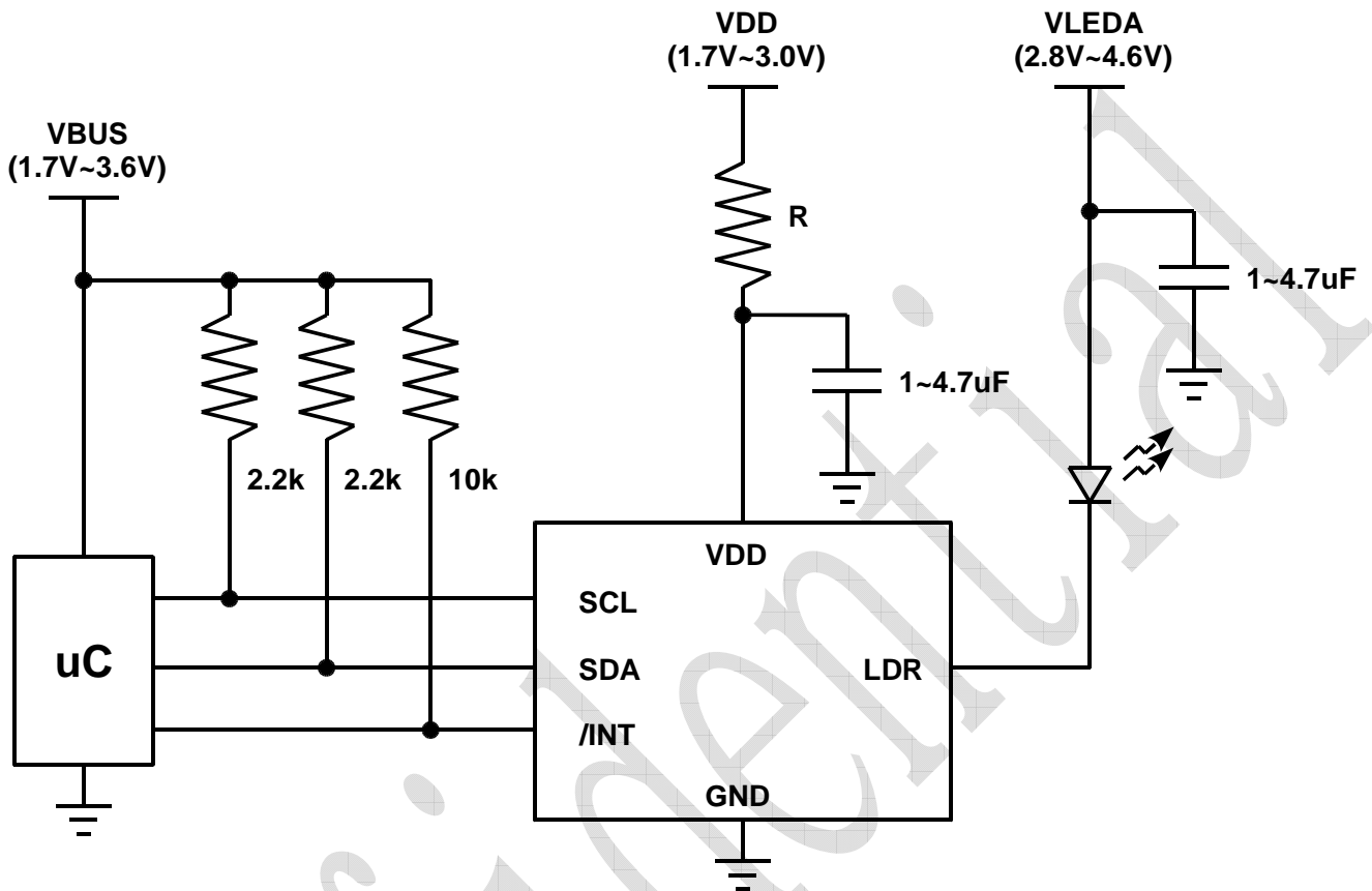
STK3232 Typical Application Circuit with Independent VDD and VLED Supply Voltage
