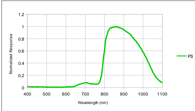
PS Spectrum
