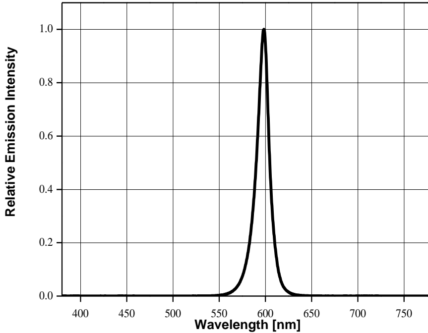
Fig 1. Color Spectrum, I_F = 140\text{mA} , T_j = 25^\circ\text{C}
