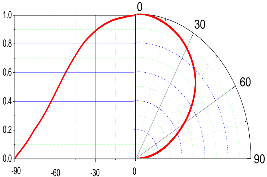
Fig 2. Viewing Angle Distribution, I_F = 140\text{mA}
