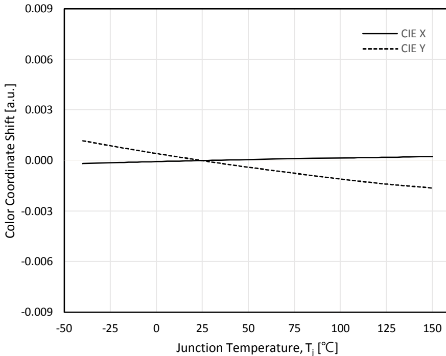
Fig 8-2. Junction Temperature vs. Color Coordinate Shift of Amber, I_F= 1.0A
