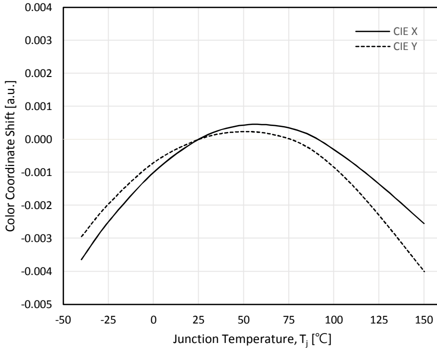
Fig 8-1. Junction Temperature vs. Color Coordinate Shift of White, I_F= 1.0A
