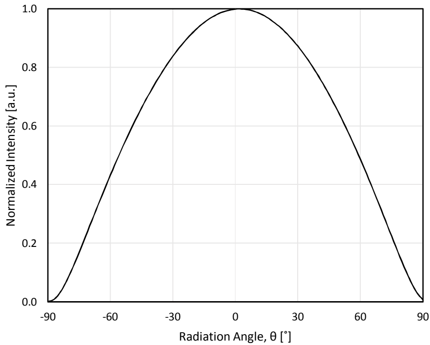
Fig 2-2. Radiant Pattern of Amber T_a = 25^\circ\text{C}
