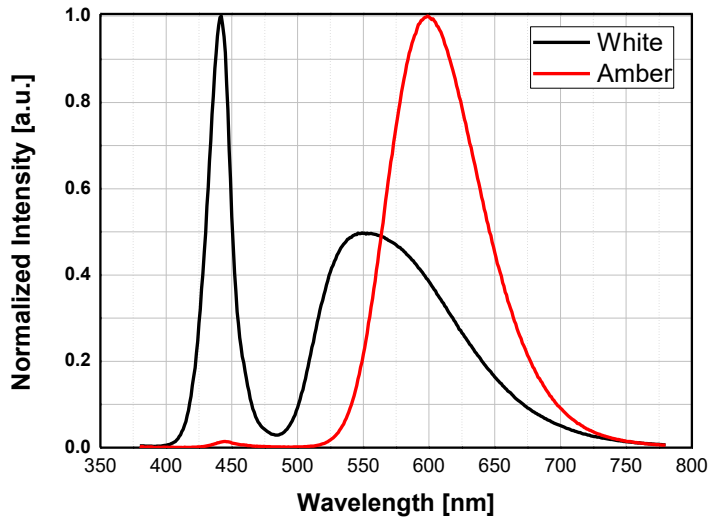
Fig 1. Color Spectrum, I_F = 0.2A , T_a = 25^\circ C
