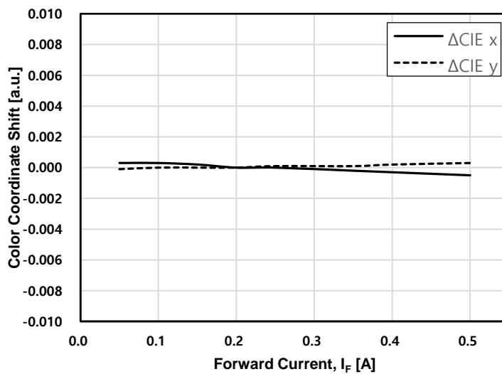
Fig 5-2. Forward Current vs. Color Coordinate Shift of amber color, T_a = 25^\circ\text{C}
