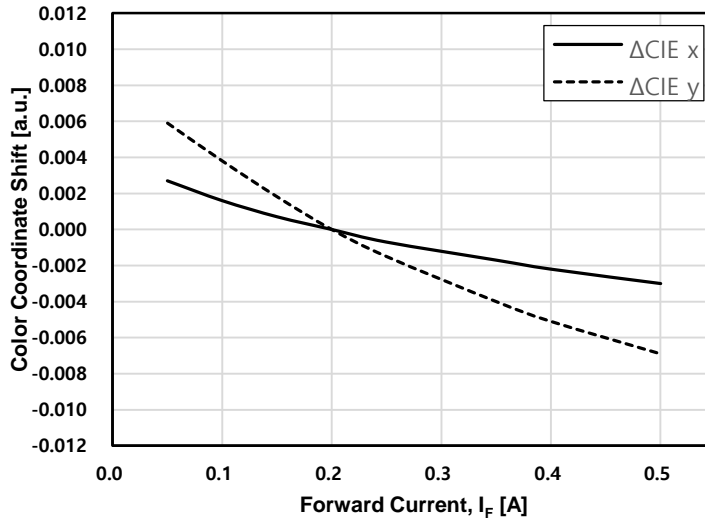
Fig 5-1. Forward Current vs. Color Coordinate Shift of white color, T_a = 25^\circ\text{C}
