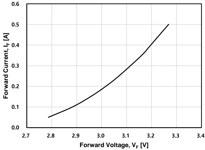
Fig 3. Forward Voltage vs. Forward Current, T_a = 25^\circ\text{C}
