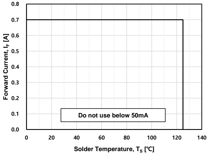
Fig 9-1. Solder Temperature vs. Allowable Forward Current. (only White ON)
