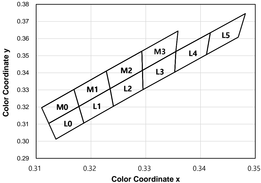
Fig 10. Color Coordinate Diagram of white color, T_a = 25^\circ\text{C} , I_F = 0.2\text{A}
