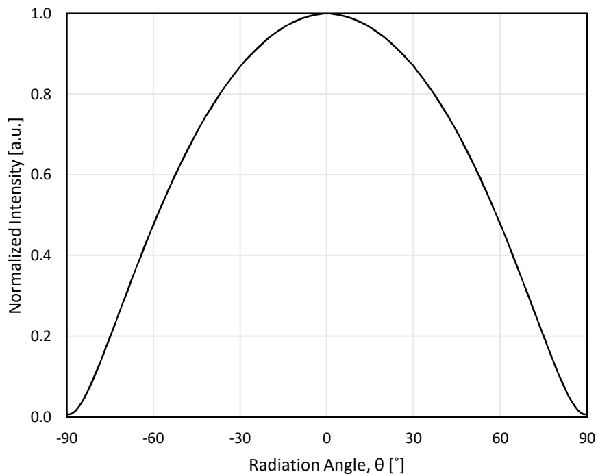
Fig 2. Radiant Pattern, T_a = 25^\circ C
