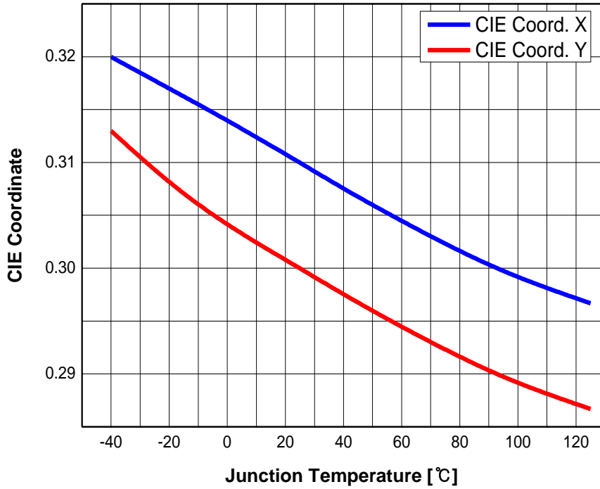
Fig 8. Chromaticity Coordinate vs. Junction Temperature, I_f = 20\text{mA}
