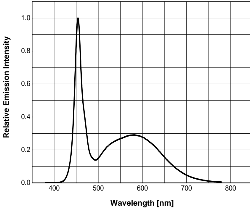
Fig 1. Color Spectrum, I_F = 20\text{mA} , T_j = 25^\circ\text{C} , RH30%
