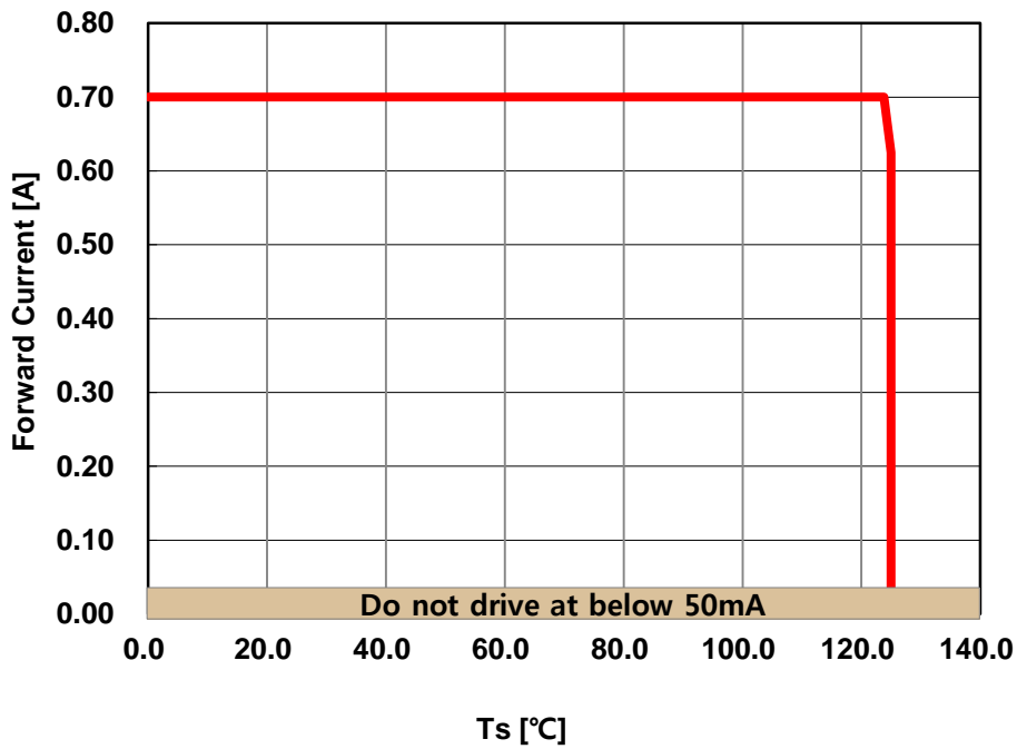
Fig 9. Maximum Forward Current vs. Solder point Temperature, T_j(\text{max.}) = 135^\circ\text{C}
