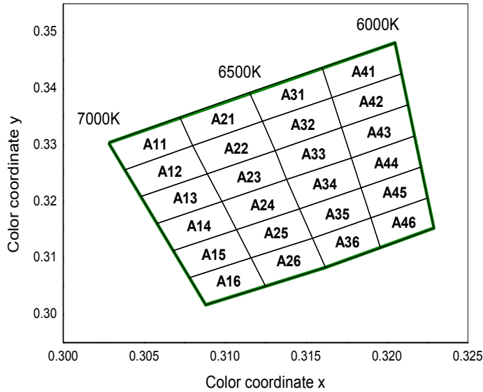
CIE Chromaticity Diagram (Cool white A), T_j=25^\circ\text{C} , I_F=65\text{mA}
