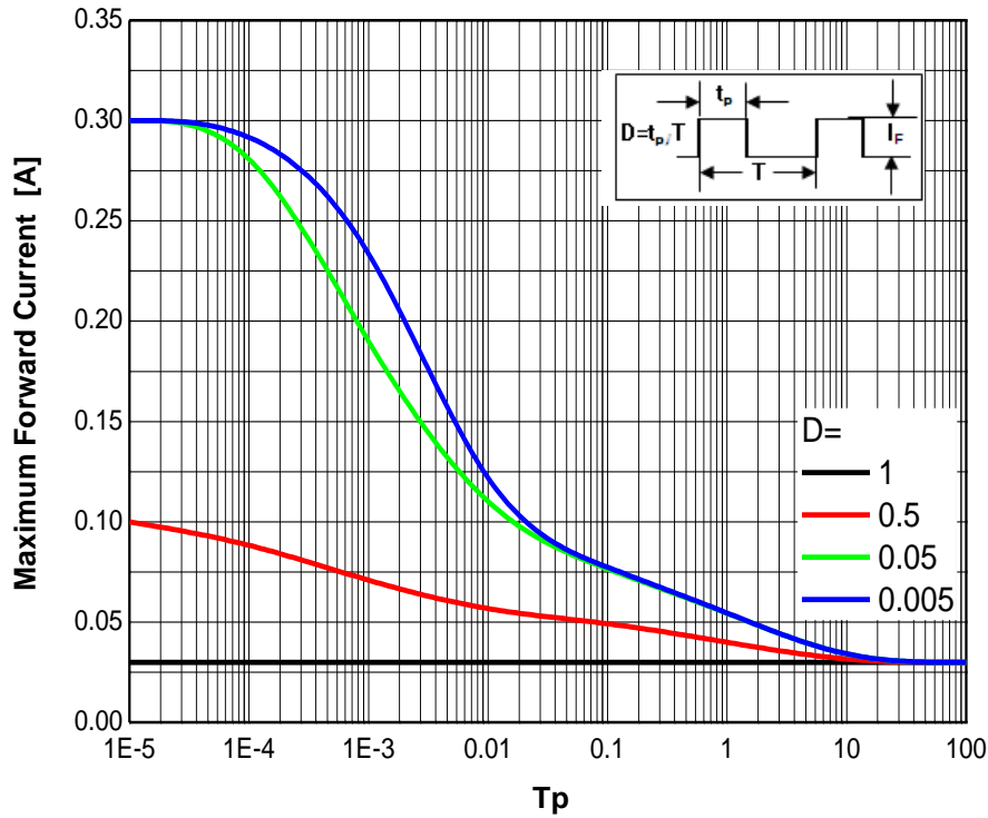
Fig 10. Maximum Forward Current vs. Duty Ratio T_j = 25^\circ\text{C}
