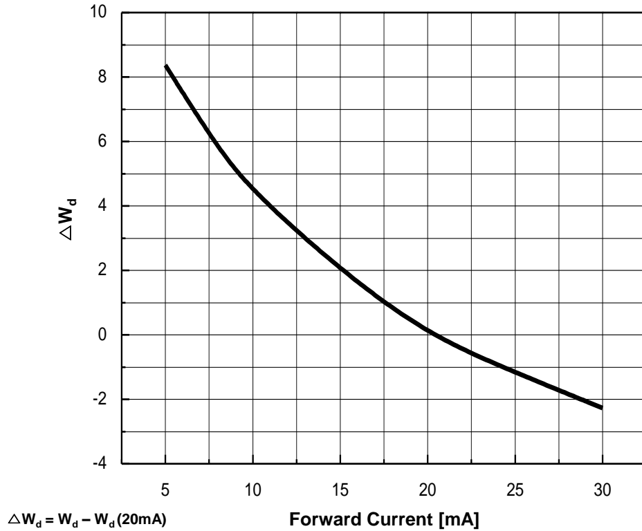
Fig 5. Forward Current vs. W_d Shift , T_j = 25^\circ\text{C}
