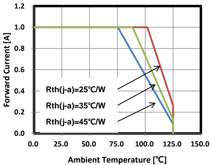
Fig 10. Maximum Forward Current vs. Ambient Temperature, T_j(\text{max.}) = 135^\circ\text{C}
