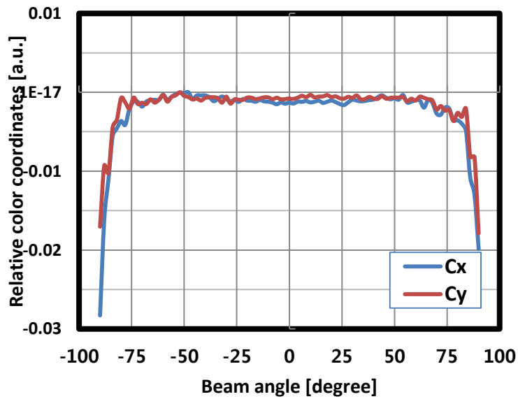
Fig 3. Distribution of color coordinates vs. Radiation Angle , T_j = 25^\circ\text{C}
