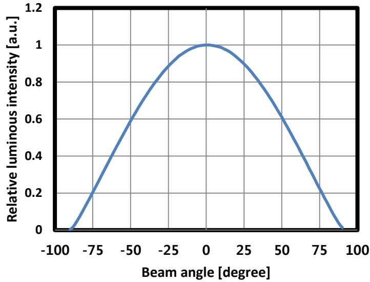
Fig 2. Relative Intensity vs. Angle, T_j = 25^\circ\text{C}
