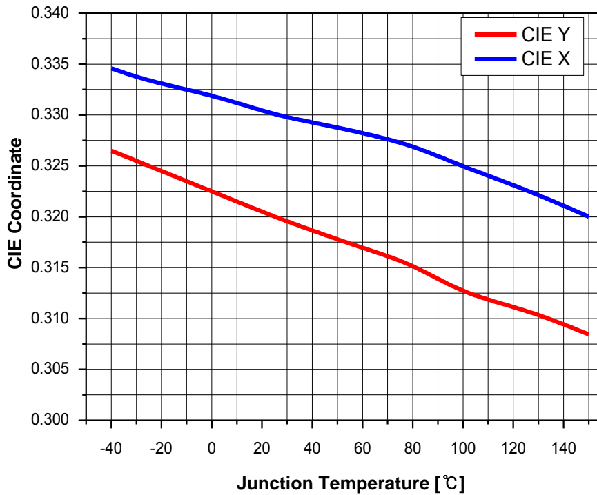
Fig 8. Chromaticity Coordinate vs. Junction Temperature, I_F = 140\text{mA}
