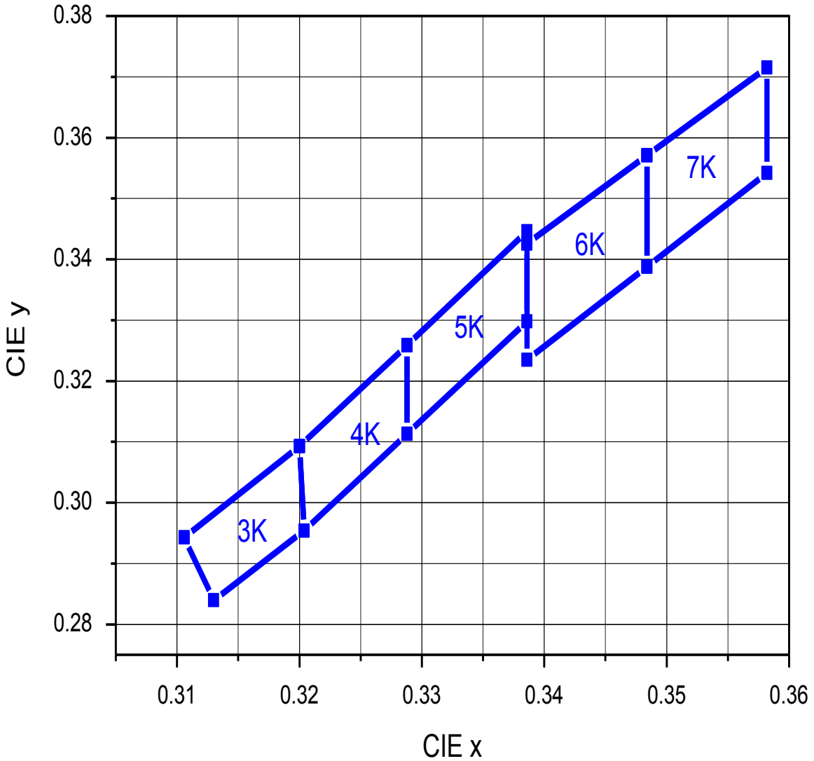
CIE Chromaticity Diagram, I_F = 140\text{mA} , T_a = 25^\circ\text{C}
