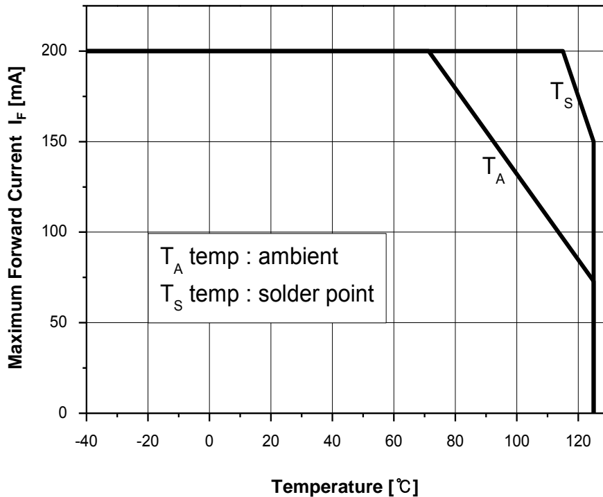
Fig 9. Maximum Forward Current vs. Temperature
