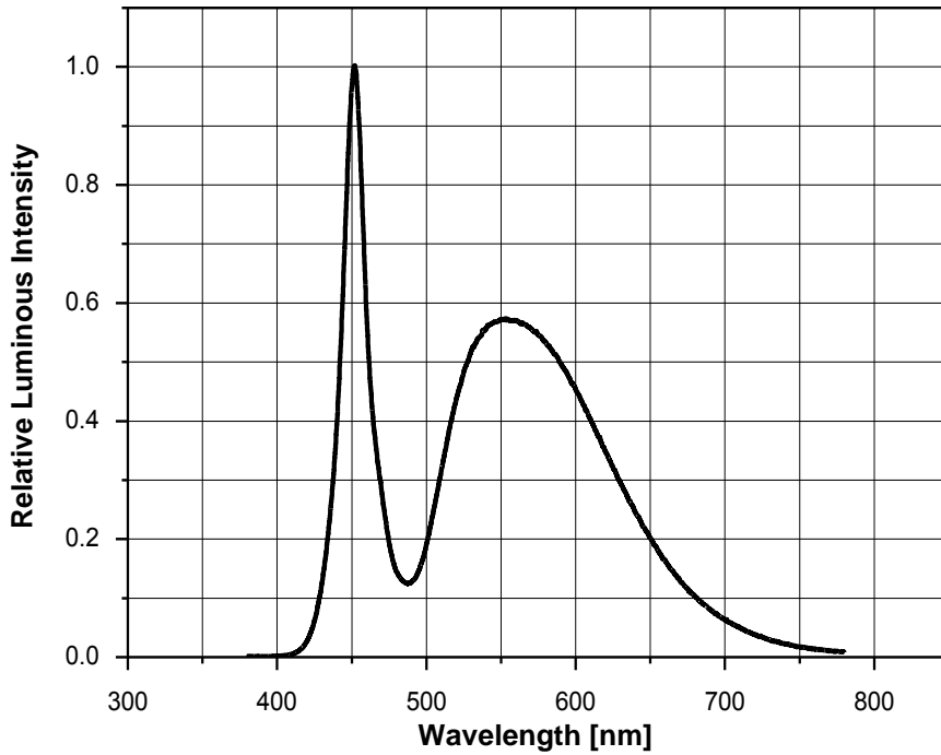
Fig 1. Color Spectrum, I_F = 140\text{mA} , T_j = 25^\circ\text{C}
