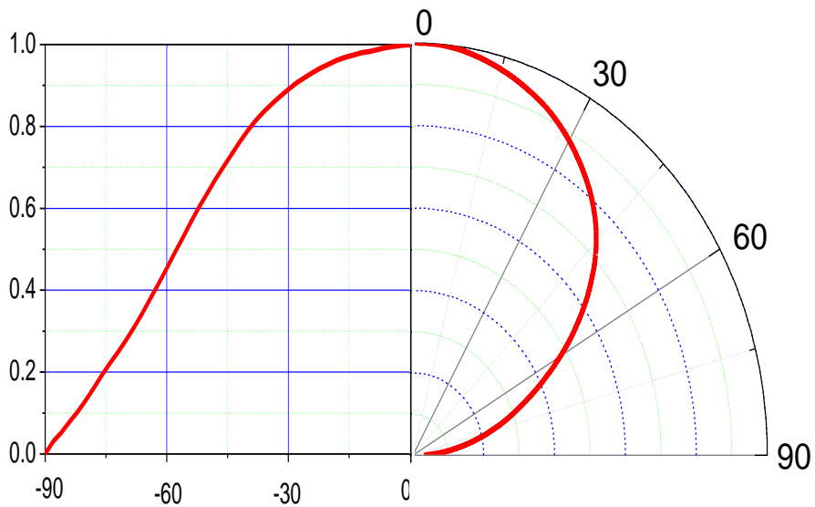
Fig 2. Viewing Angle Distribution, I_F = 140\text{mA}
