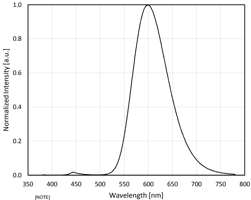
Fig 1. Color Spectrum, I_F = 1.0A , T_a = 25^\circ C
