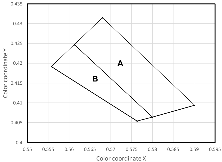
Fig 10. Color Coordinate Diagram, T_a = 25^\circ\text{C} , I_F = 1.0\text{A}
