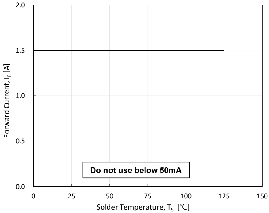
Fig 9. Solder Temperature vs. Allowable Forward Current
