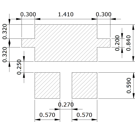
Solder Pad
