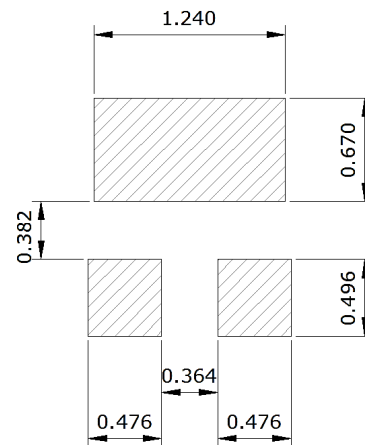
Solder Metal Mask
