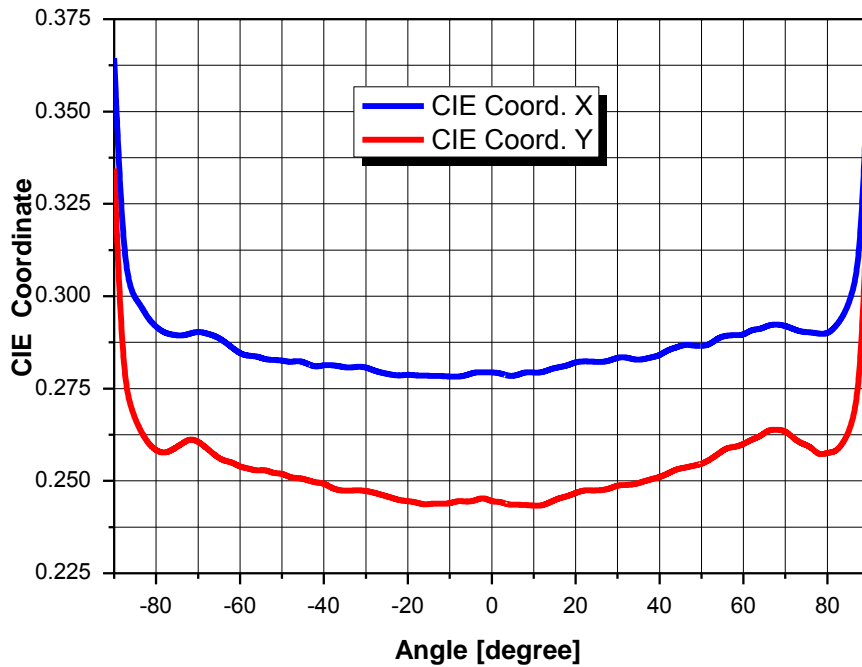
Fig 10. Color vs. Viewing Angle, I_F = 10\text{mA} , T_j = 25^\circ\text{C}
