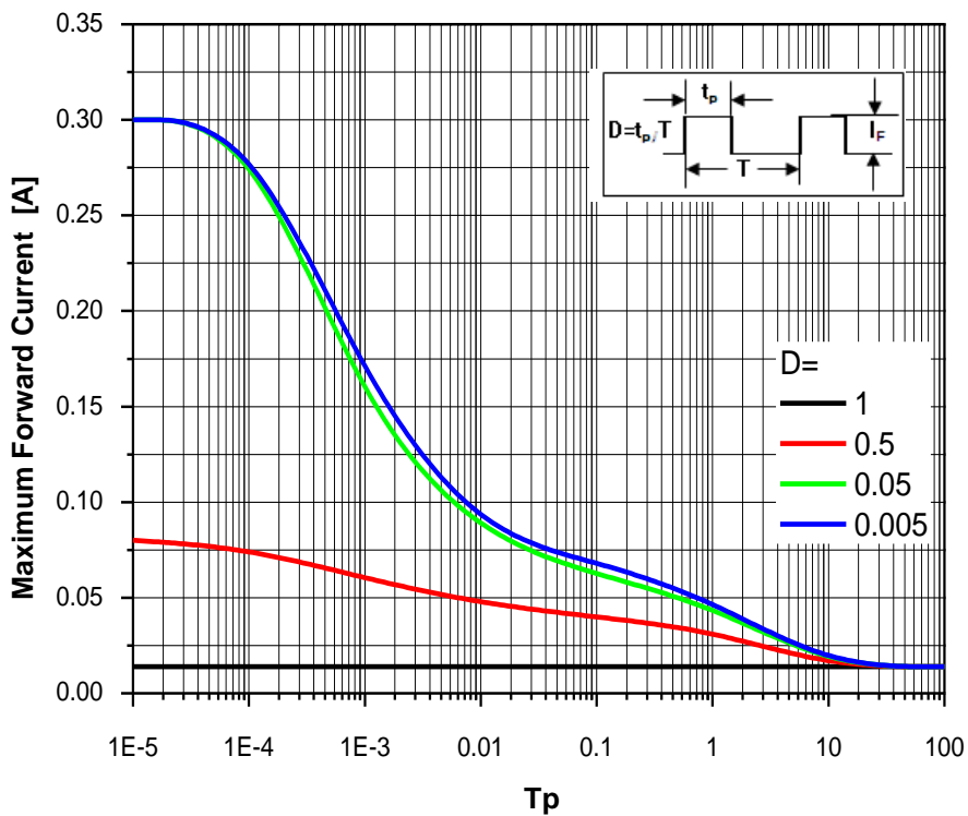
Fig 12. Maximum Forward Current vs. Duty Ratio T_j = 85^\circ\text{C}
