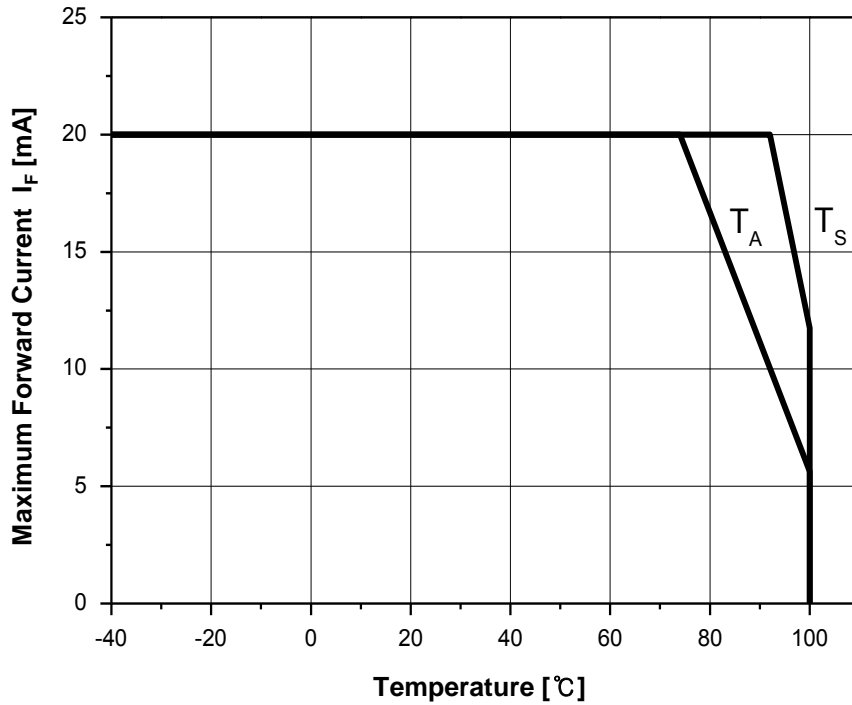
Fig 9. Maximum Forward Current vs. Temperature
