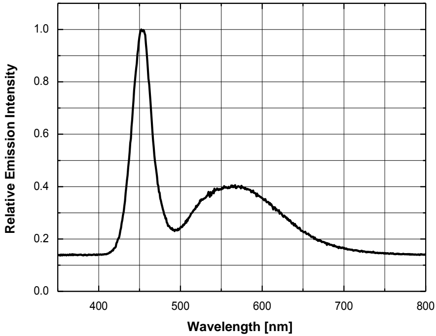
Fig 1. Color Spectrum, I_F = 10\text{mA} , T_j = 25^\circ\text{C} , RH30%
