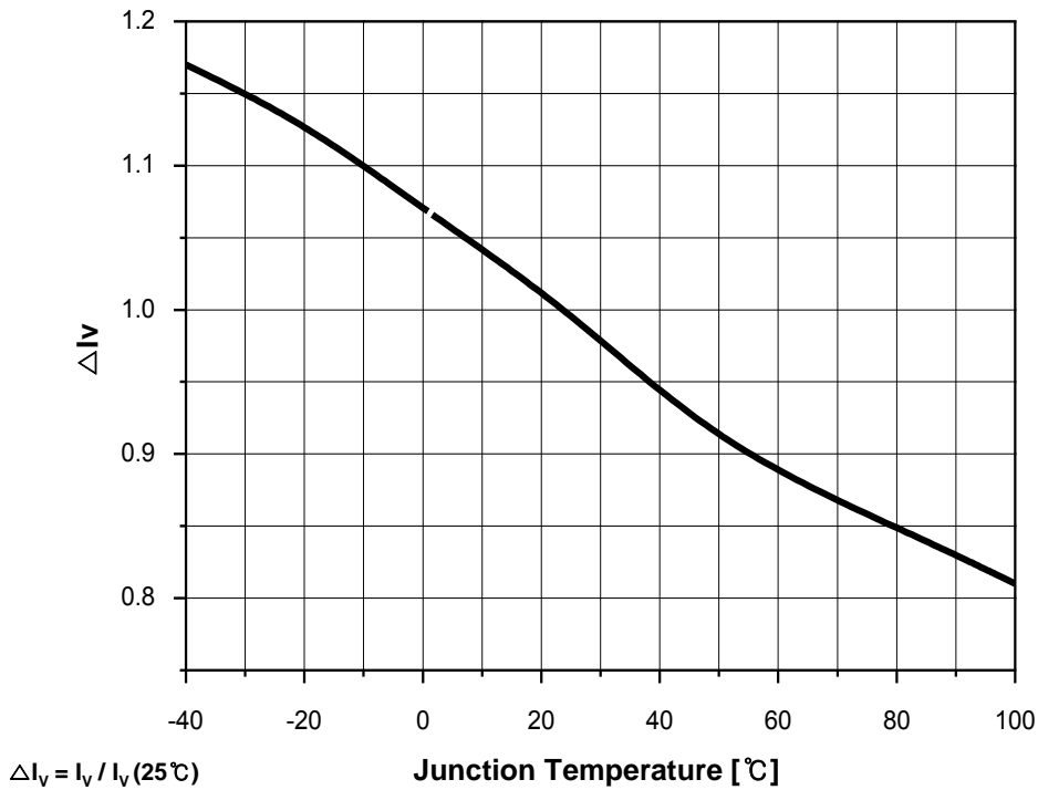
Fig 6. Relative Light Output vs. Junction Temperature, I_F = 10\text{mA}
