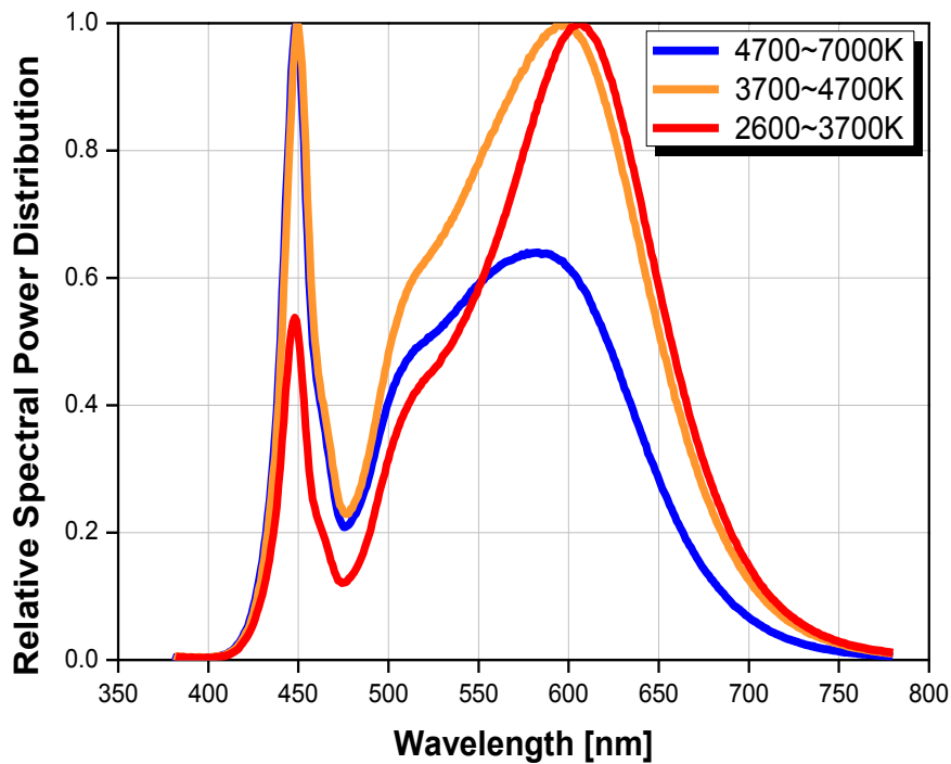
Fig 1. Color Spectrum, T_j=25^\circ\text{C} , I_F=640\text{mA} (CRI80)
