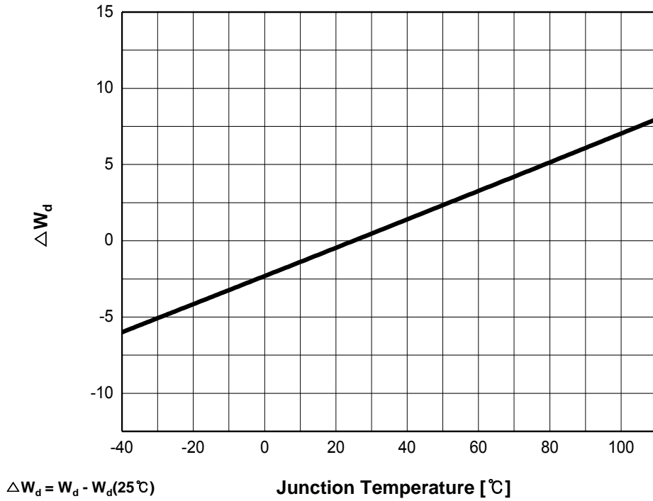
Fig 8. Dominant wavelength shift vs. Junction Temperature, I_F = 10\text{mA}
