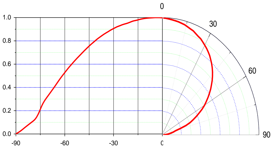
Fig 2. Viewing Angle Distribution, I_F = 10\text{mA}
