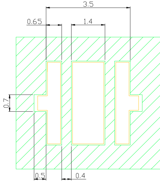
Solder Resist
