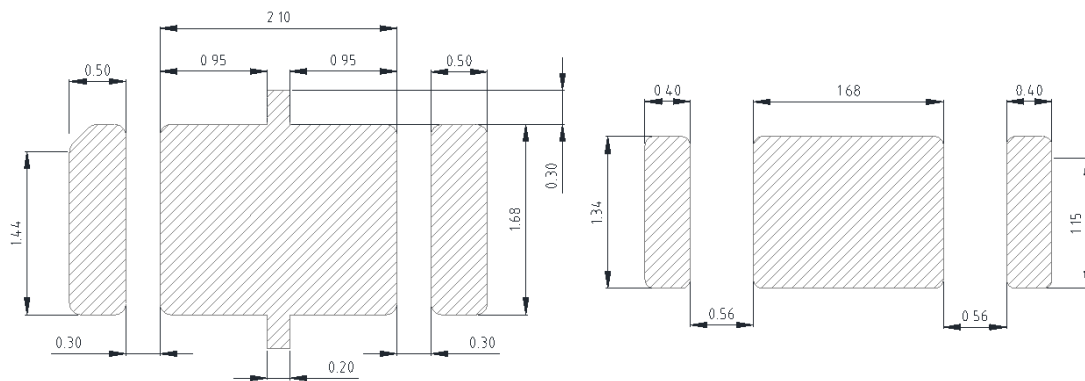
< Solder Pad >
