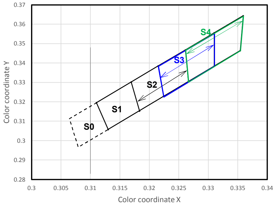
Fig 10. Color Coordinate Diagram, T_a = 25^\circ\text{C} , I_F = 1.0\text{A}
