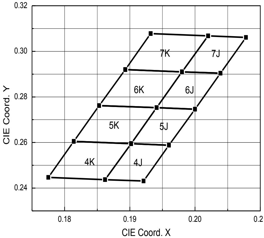
CIE Chromaticity Diagram, I_F = 20\text{mA} , T_j = 25^\circ\text{C}
