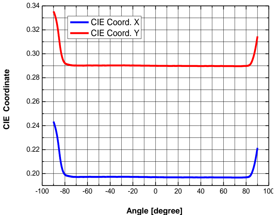
Fig 10. Color. vs. Viewing Angle, T_j = 25^\circ\text{C} , I_F = 20\text{mA}
