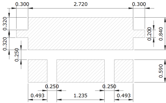
Solder Pad
