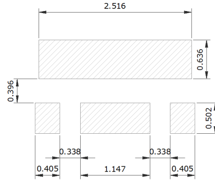
Solder Metal Mask
