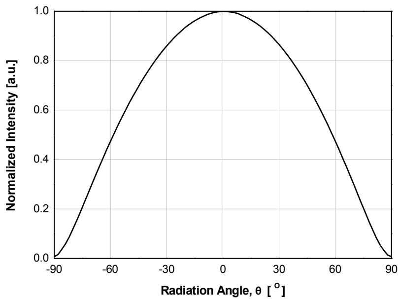
Fig 2. Radiant Pattern, T_a = 25^\circ C
