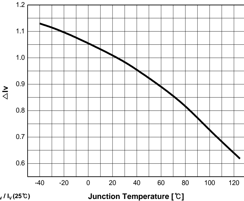
Fig 6. Relative Light Output vs. Junction Temperature, I_F = 20\text{mA}
