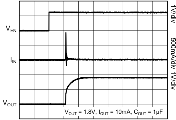
Time (50 \mu\text{s}/\text{div} )
