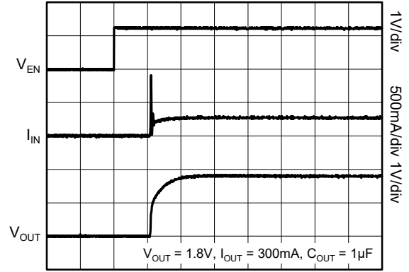
Time (50 \mu\text{s}/\text{div} )
