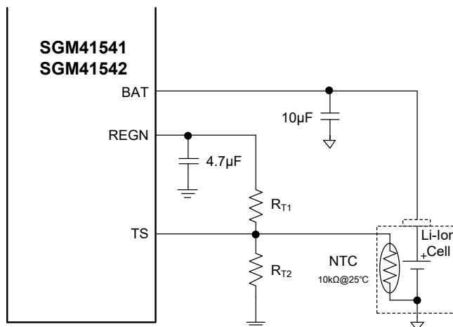
Figure 6. Battery Thermistor Connection and Bias Network
