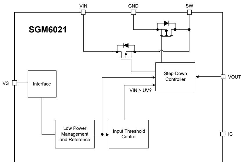
Figure 2. Block Diagram
