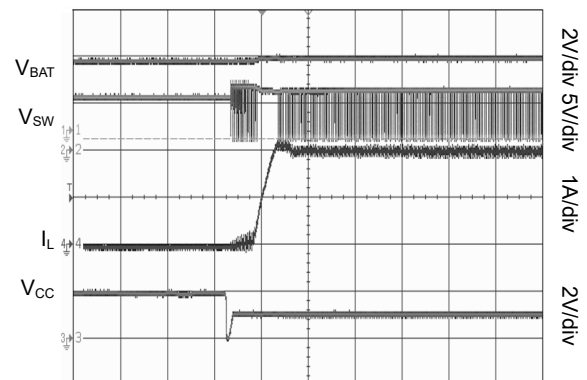
Time (20μs/div)
