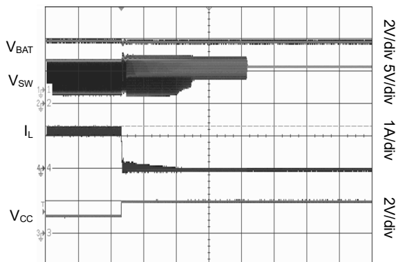
Time (50μs/div)
