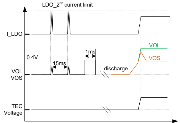
Figure 9. Hiccup Mode Protection
