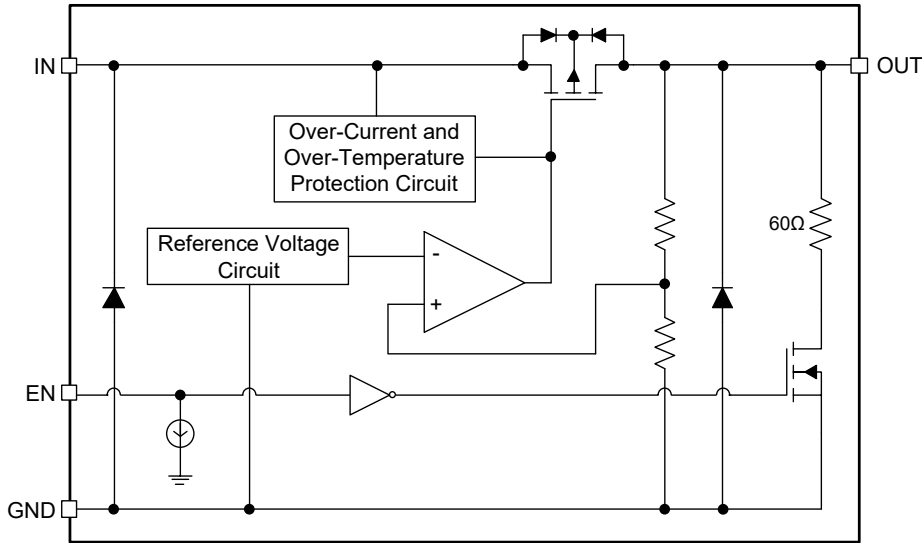
Figure 2. Block Diagram
