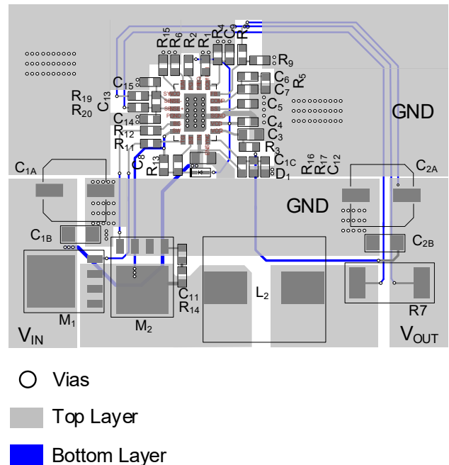
Figure 10. Layout Example
