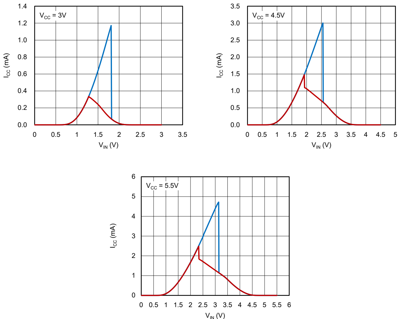
Figure 1. Typical Transfer Characteristics
