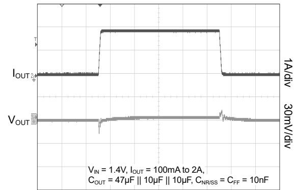
Time (200µs/div)
