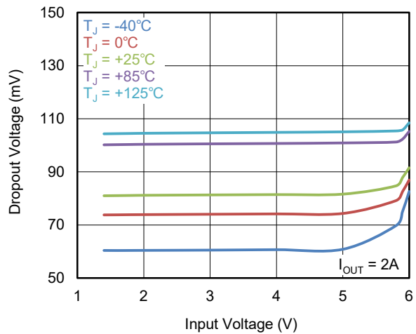
Dropout Voltage vs. Input Voltage without BIAS
