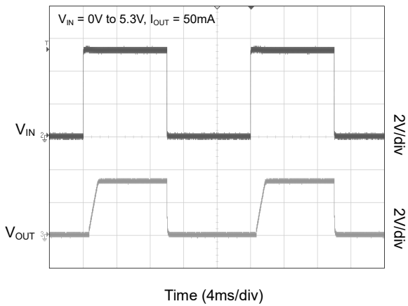
Power-Up/Power-Down Output Waveform
