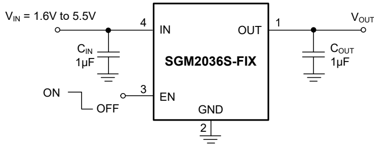
Figure 4. Fixed Output Version (XTDFN-1x1-4L)
