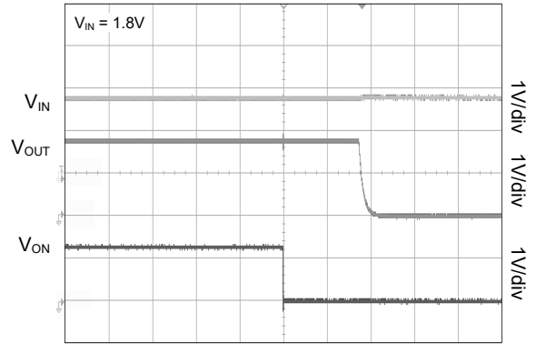
Time (10μs/div)
