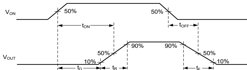
Figure 3. Timing Waveforms
