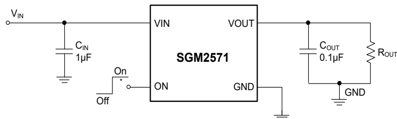
Figure 2. Test Circuit
