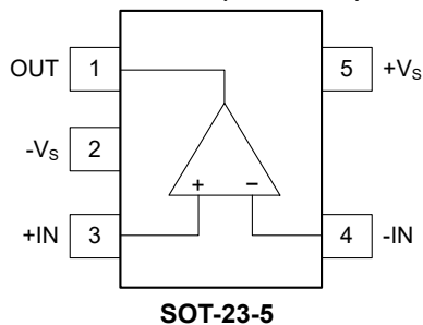
SGM8969-1 (TOP VIEW)
