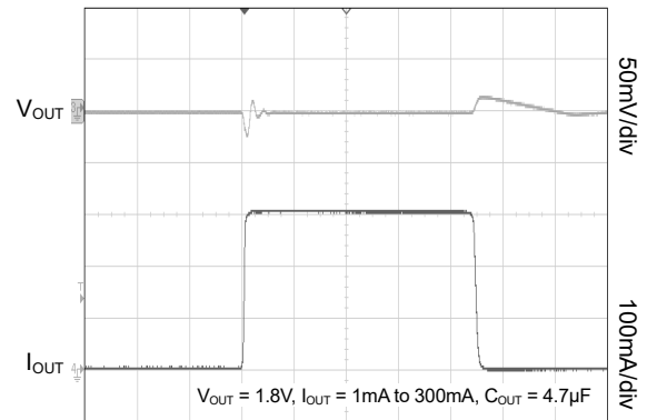
Time (10 \mu\text{s/div} )
