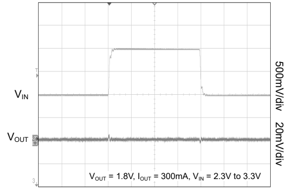
Time (20 \mu\text{s/div} )
