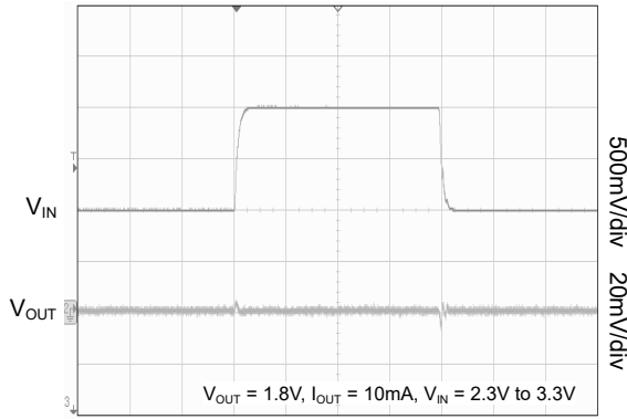
Time (20 \mu\text{s/div} )
