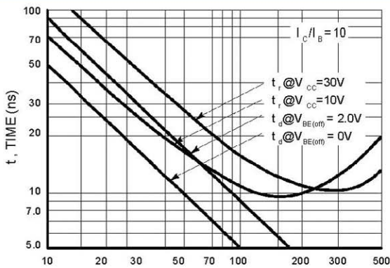
Figure 5. Turn-On Time
