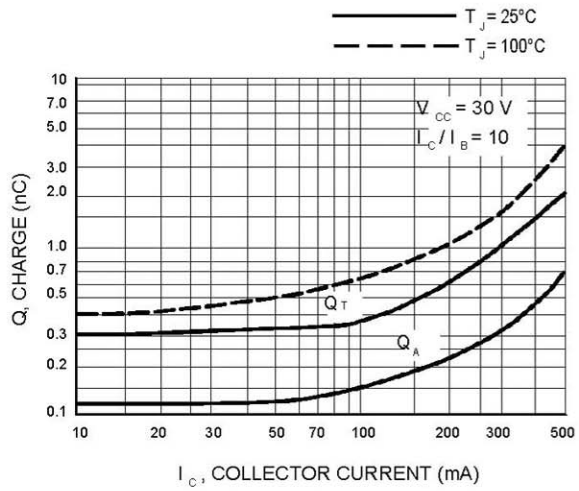
Figure 4. Charge Data
