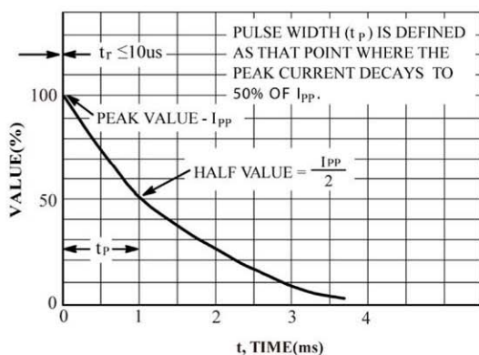
FIG.5 Pulse Waveform
