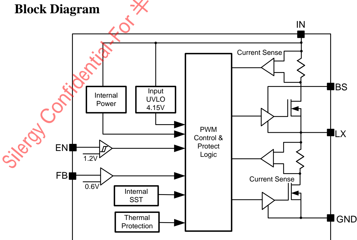
Figure3. Block Diagram
