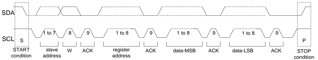
Figure 35. Write Sequence
