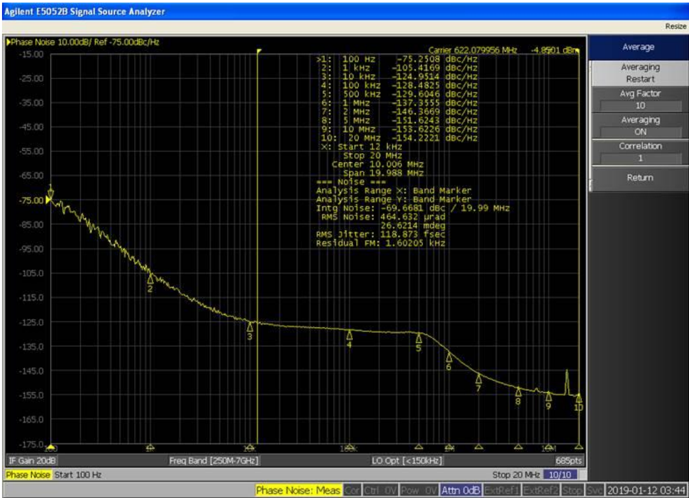
Figure 2. Representative Phase Noise Measurement: F_{OUT} = 622.08\text{ MHz} , F_{IN} = 10\text{ MHz} , BW = 100 Hz
