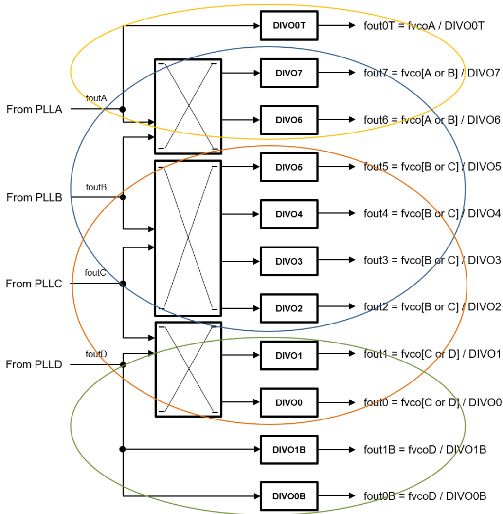
Figure 10. Output Clock Distribution
