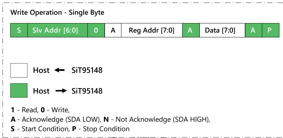
Figure 34. Write Block
