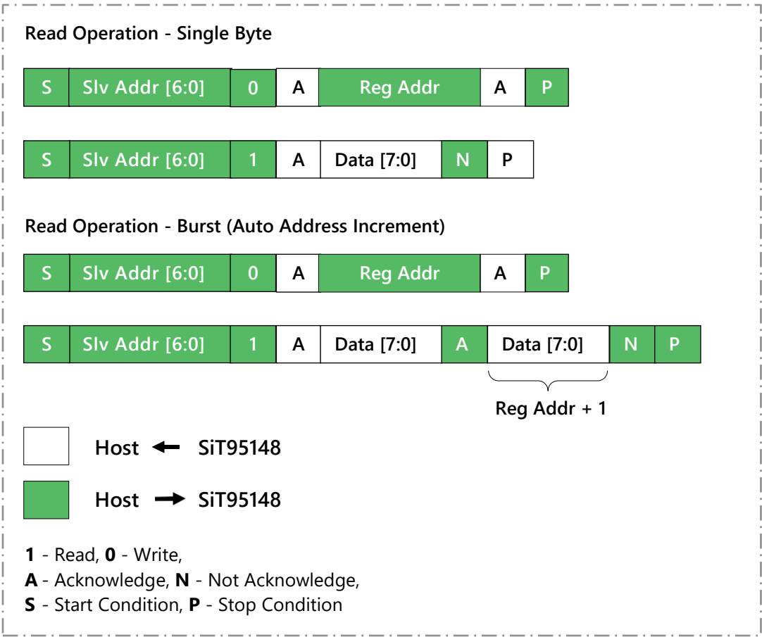
Figure 33. Read Block
