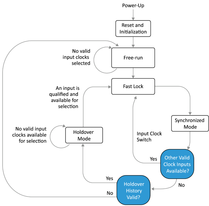
Figure 15. Operation Modes
