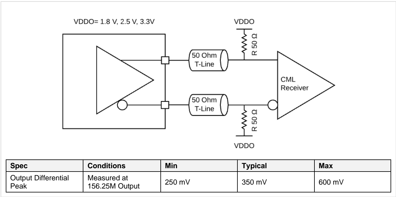
Figure 28. CML Interface Termination
