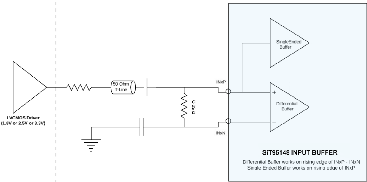
Figure 19. AC Coupled Single Ended Driver with 50 \Omega Termination on receiver (chip) side
