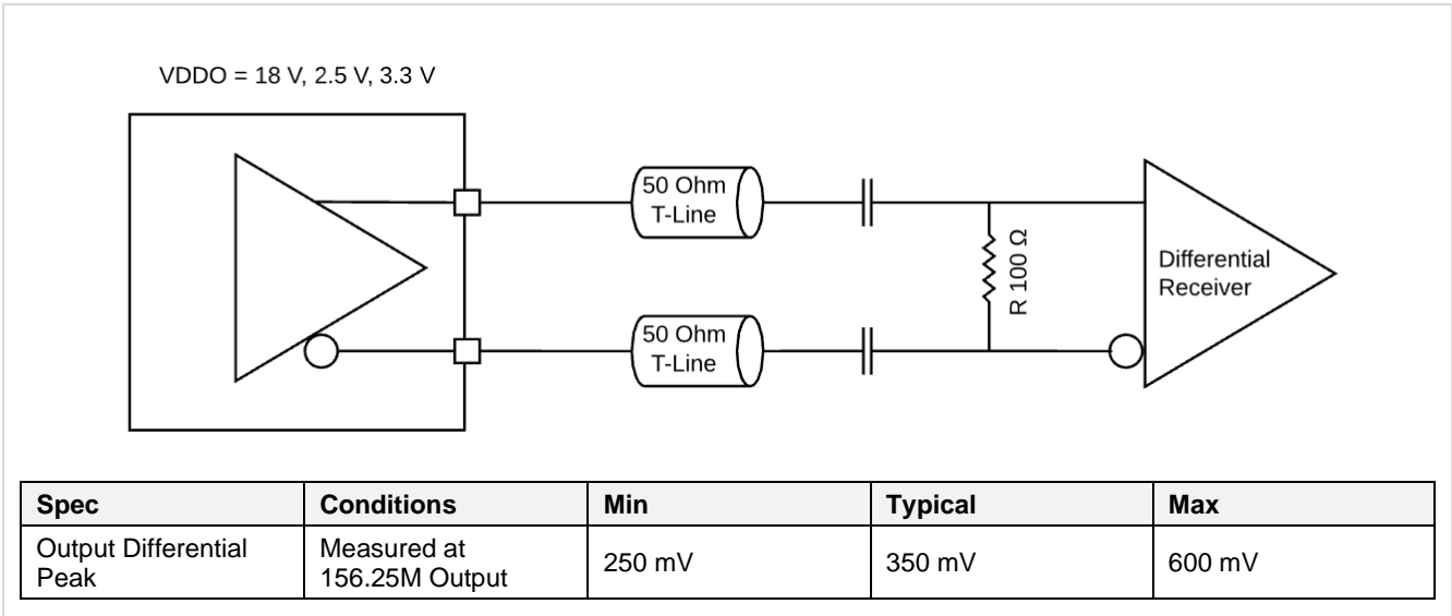
Figure 25. LVDS AC Termination at the Load
