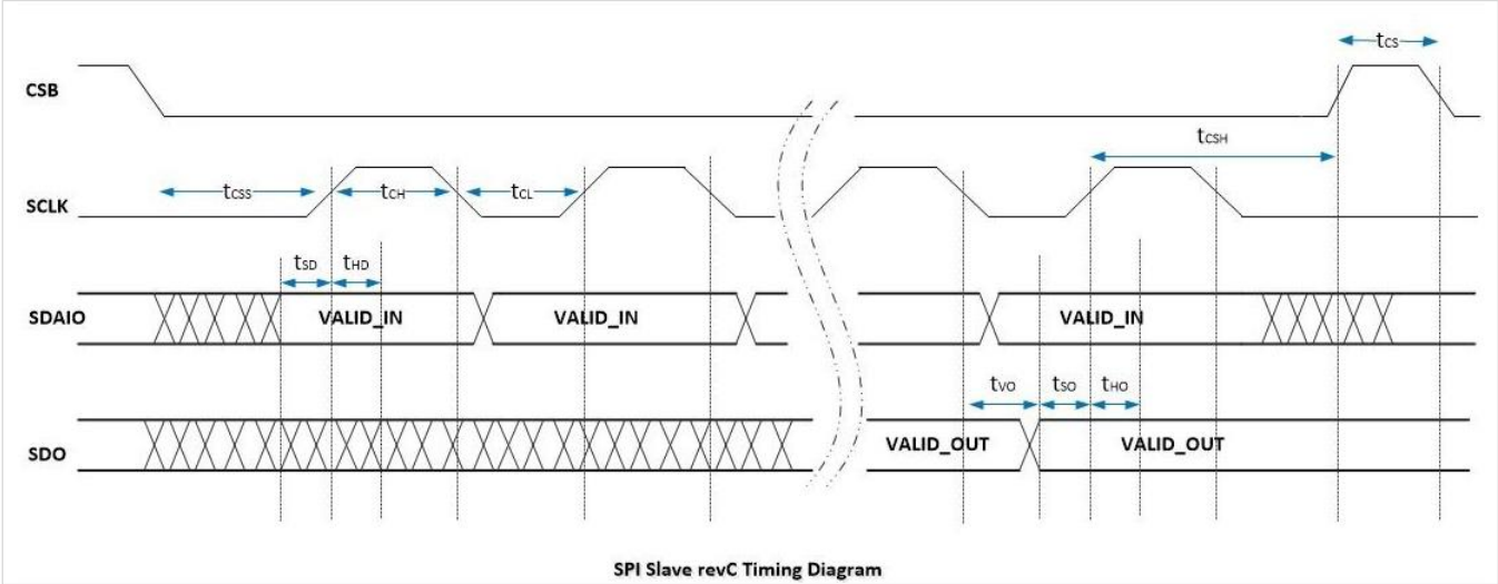
Figure 35. SPI Timing Diagram
