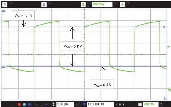
Figure 3. SiT1552AI-JE-D14-32.768 Output Waveform (10 pF load)
